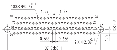
J30JZ/XLN(S) 100TJWA000
