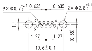
J30JZ/XPn(S) 9TJNAP01
