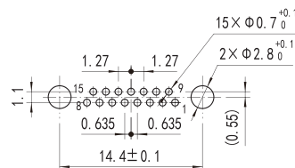
J30JZ/XPn(S) 15TJNAP01
