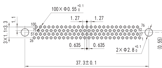
J30JZ/XPn(S) 100TJNAP01
