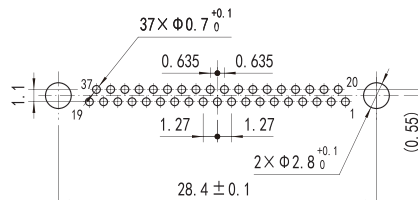
J30JZ/XPn(S) 66TJNAP01
