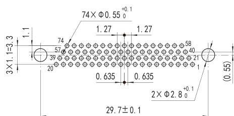
J30JZ/XPn(S) 74TJNAP01
