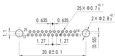
J30JZ/XPn(S) 25TJNAP01
