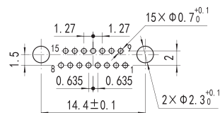
J30JZ/XLN(S) 15TJWA000
