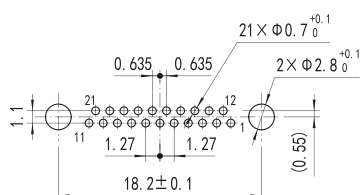
J30JZ/XPn(S) 21TJNAP01
