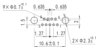
J30JZ/XLN(S) 9TJWA000
