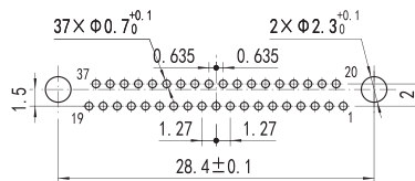
J30JZ/XLN(S) 37TJWA000
